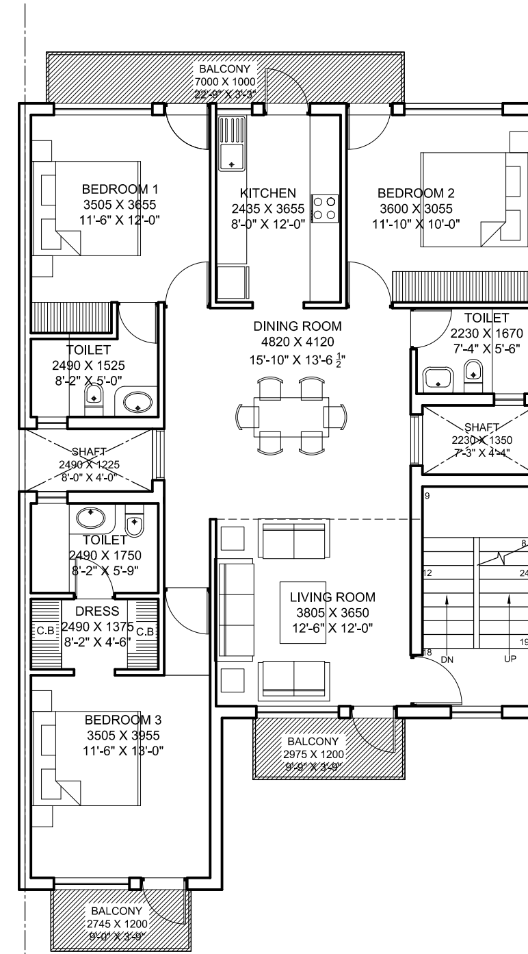
FIRST FLOOR PLAN REVISED OPTION
