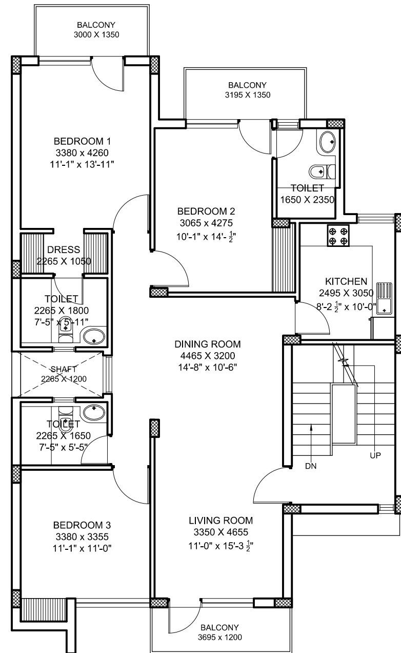
FIRST FLOOR PLAN ORIGINAL OPTION
