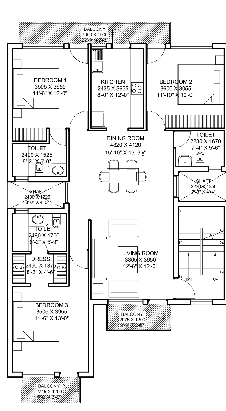
SECOND FLOOR PLAN REVISED OPTION
