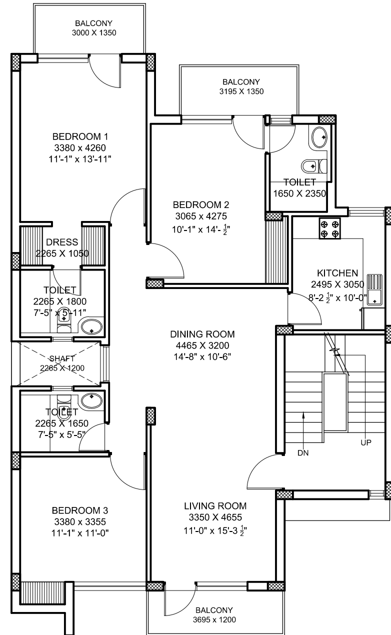
SECOND FLOOR PLAN ORIGINAL OPTION
