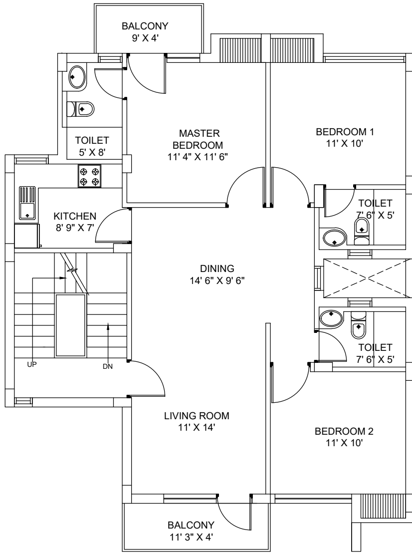
TYPICAL FLOOR PLAN ORIGINAL OPTION
